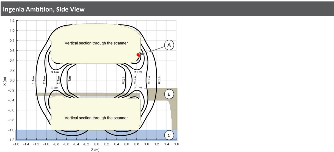
Fig. 4: Side View, vertical section: Spatial gradient of static magnet field B_0
