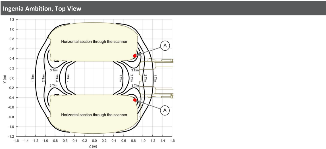
Fig. 3: Top View, horizontal section: Spatial gradient of static magnet field B_0
